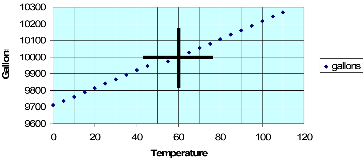
Gasoline Temperature Expansion
